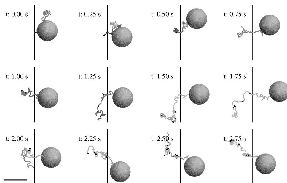
Figure 5. The uptake of a DNA filament. Its length is 8\ \mu\text{m} , the bond length is b = 100\ \text{nm} and the radius of the polystyrene bead is R_b = 500\ \text{nm} . The black dots represent occupied binding sites. The horizontal bar in the bottom left corner corresponds to 1\ \mu\text{m} . The grey scale indicates the position in the third dimension (depth).
